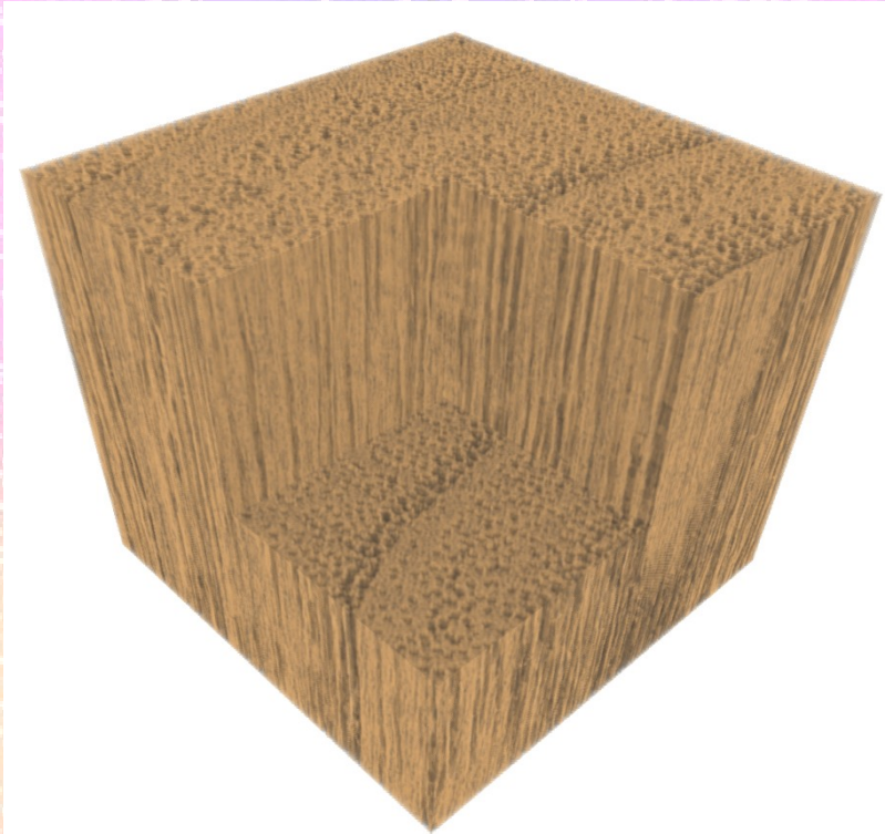
Tomographic reconstruction
